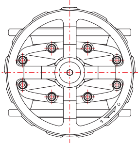
Handwheel
